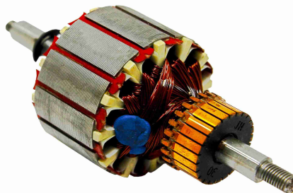
RLB-3000 REF A 27.23 PZA |INDUCIDO(ROTOR) P/LICUADORA OSTER
