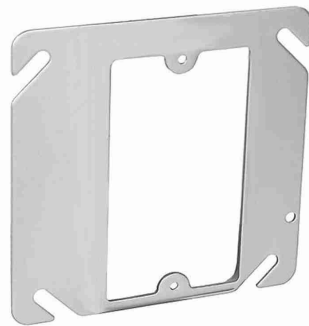
EMT-4930 REF C 1.39 PZA |MARCO REDUCTOR MET 4X4 A 2X4 LISO REF A=0.87 REF B=1.32
