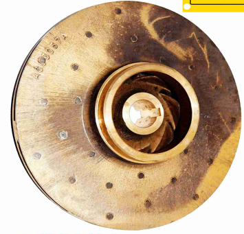
AHD-4527 REF C 218.1 PZA | IMPELLER BRONCE CP680C 5.5H PEDROL REF A=136.14 REF B=207.21
