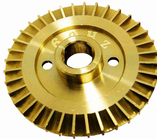
AHD-4517 REF C 20.72 PZA | IMPEL.B/A PKM60 1/2"S/CHAVETERO PED REF A=12.93 REF B=19.68
